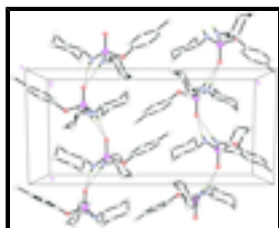
Fig. 2. A view of the crystal packing showing the formation of chains through N—H...O hydrogen bonds (shown as dashed lines). H atoms not involved in hydrogen bonding have been omitted for clarity.
